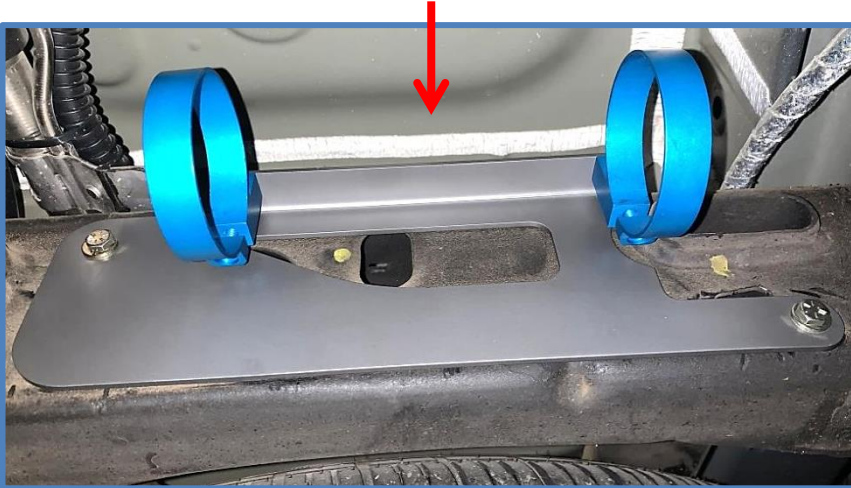
Left reservoir bracket installed with provided hardware.
